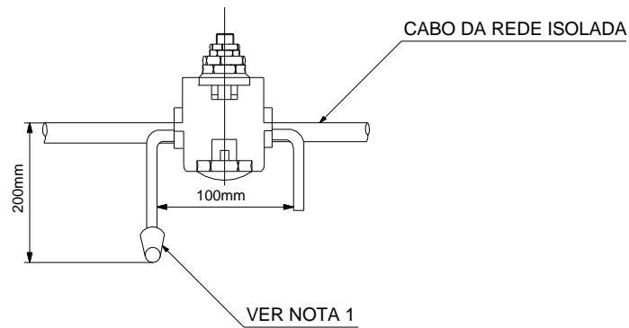
Figura 54 – Conexões – Conector piercing
